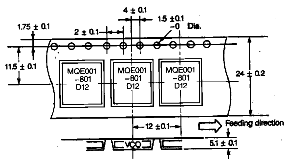
Taping Specifications: mm
